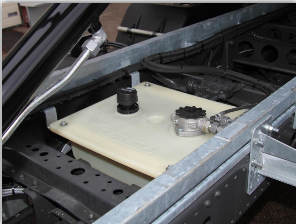
RESERVOIR HYDRAULIQUE POLYETHYLENE / HYDRAULIC TANK POLYETHYLENE
